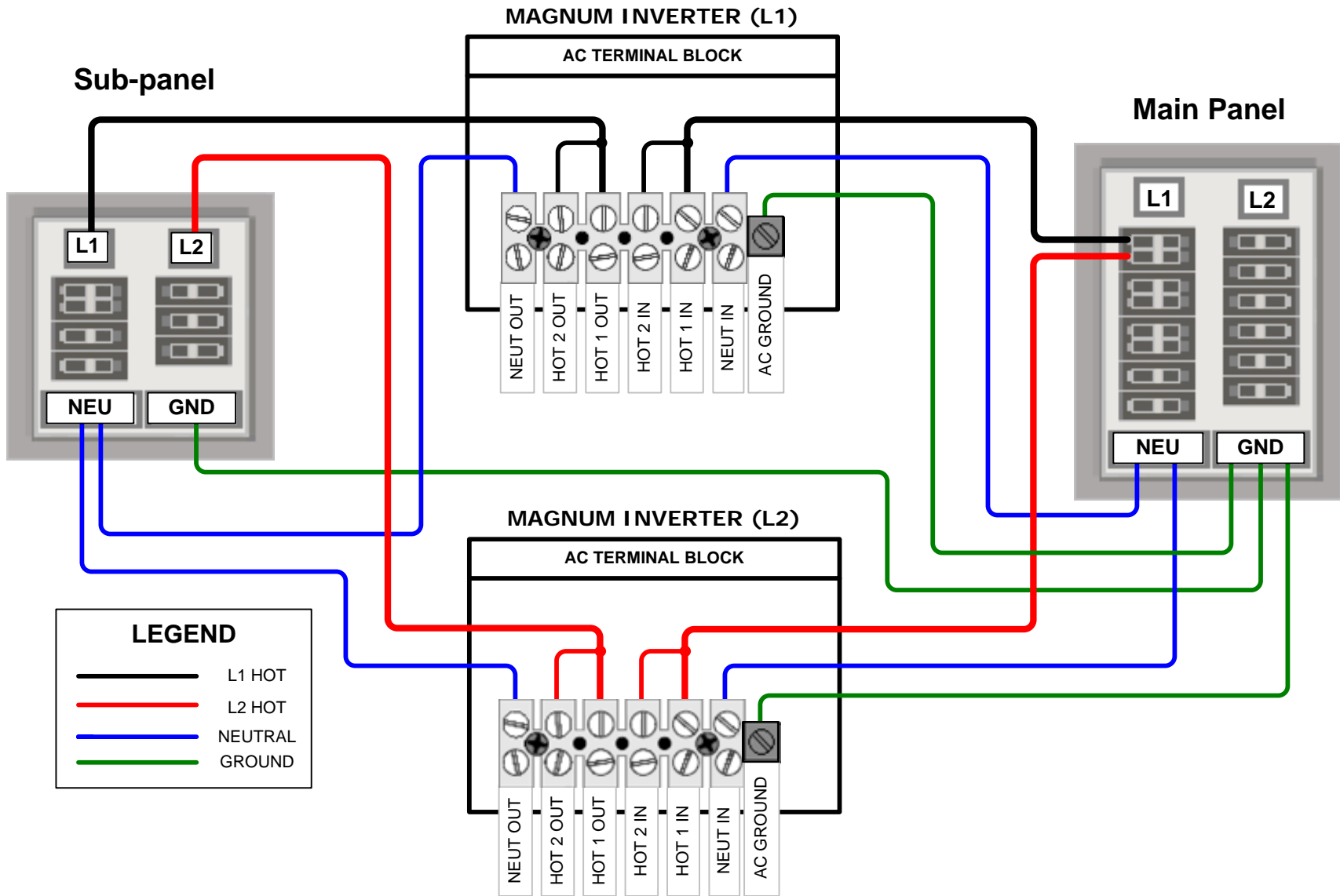
Single In/Single Out (60A with 120/240VAC source)
